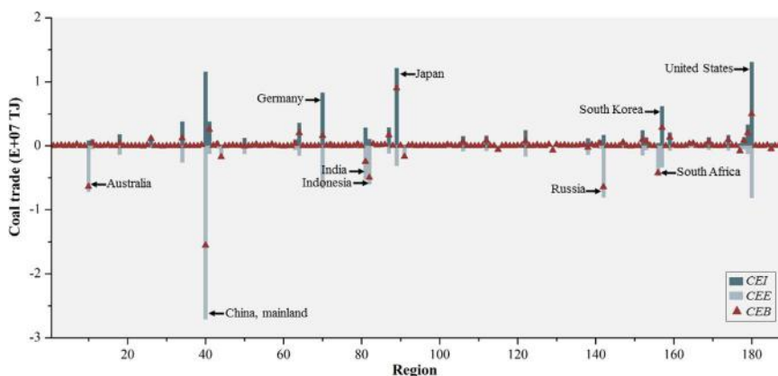
Fig. 6. CEI (coal embodied in imports), CEE (coal embodied in exports) and CEB (coal embodied in trade balance) of the 188 regions (See Appendix A for details of the regions.).
